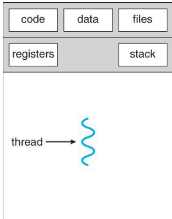
single-threaded process
