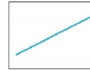
Aliasing
