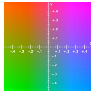
U-V Color Plane
