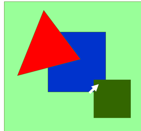
Front-buffer
