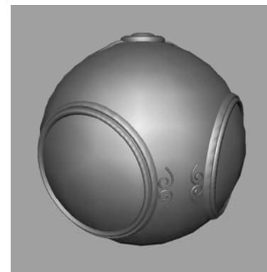
geometric model
