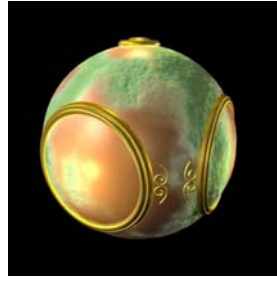
Bump mapping
