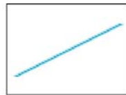
Anti-aliased
