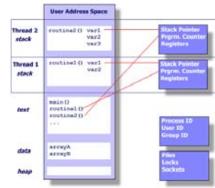
THREADS WITHIN A UNIX PROCESS
